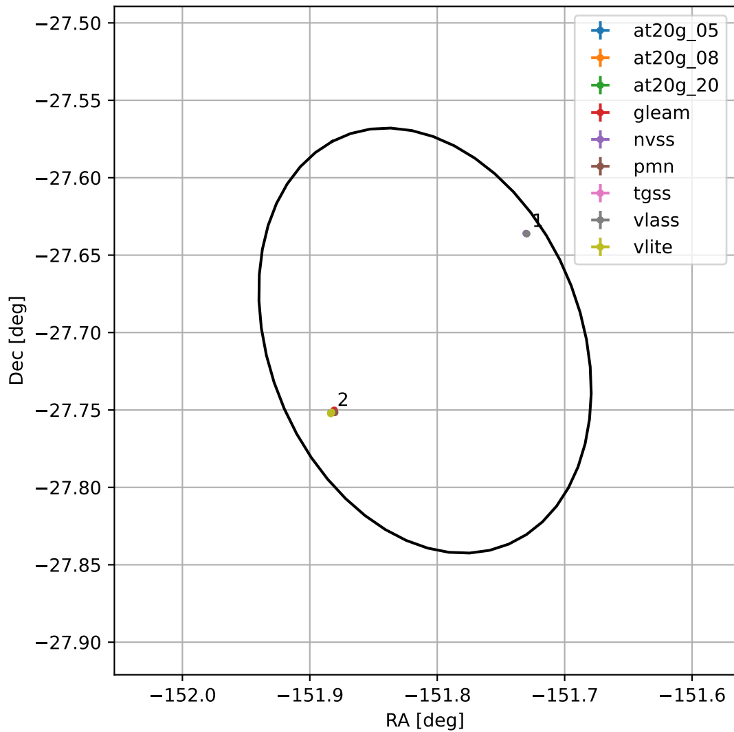
4FGL J1352.7-2742
