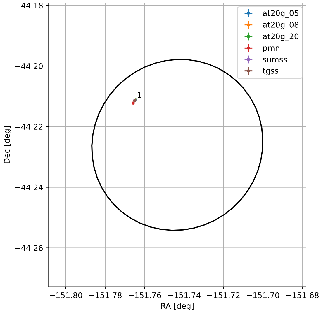
4FGL J1353.0-4413
