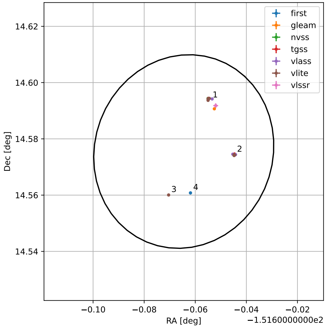
4FGL J1353.3+1434
