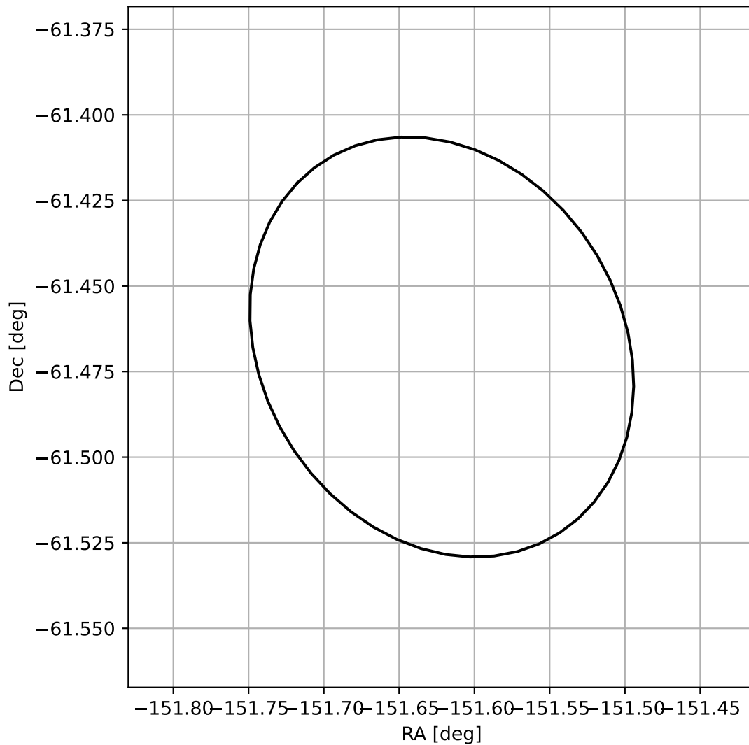
4FGL J1353.5-6128
