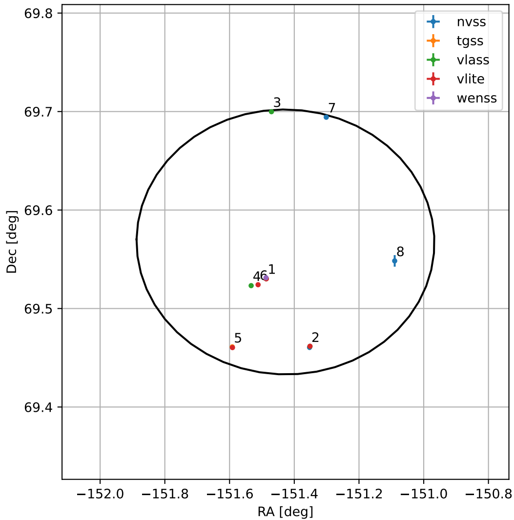
4FGL J1354.2+6934
