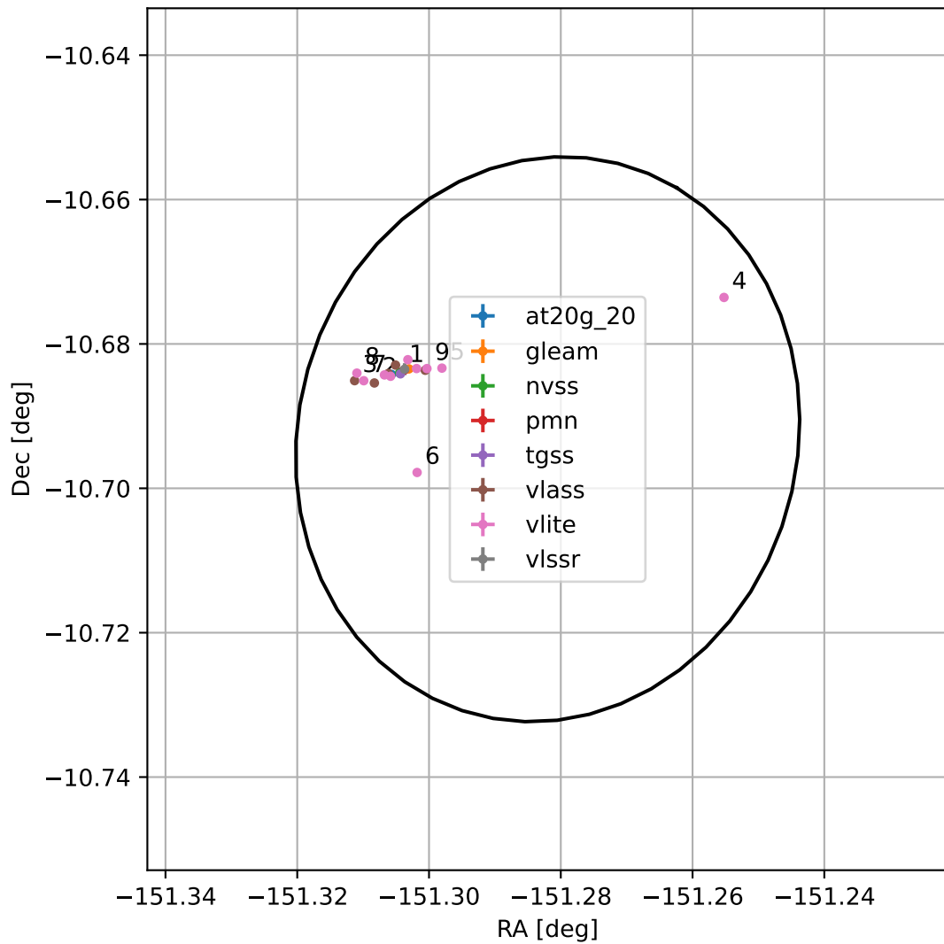
4FGL J1354.8-1041
