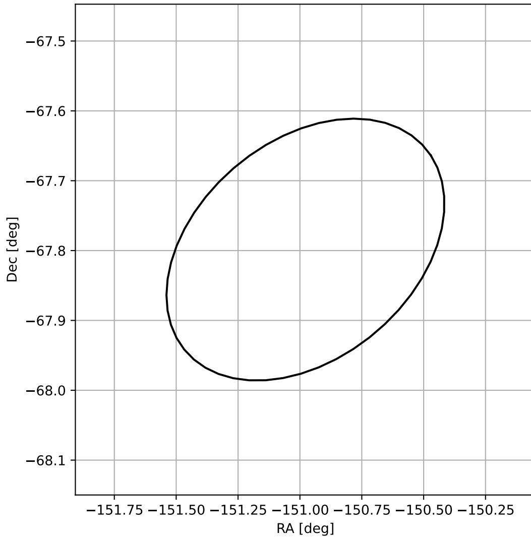
4FGL J1356.0-6747
