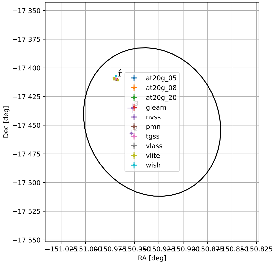
4FGL J1356.2-1726
