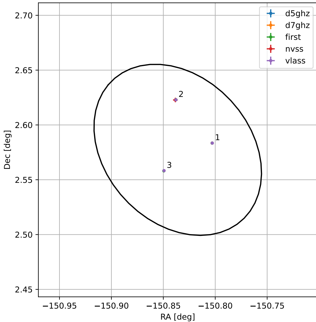
4FGL J1356.6+0234
