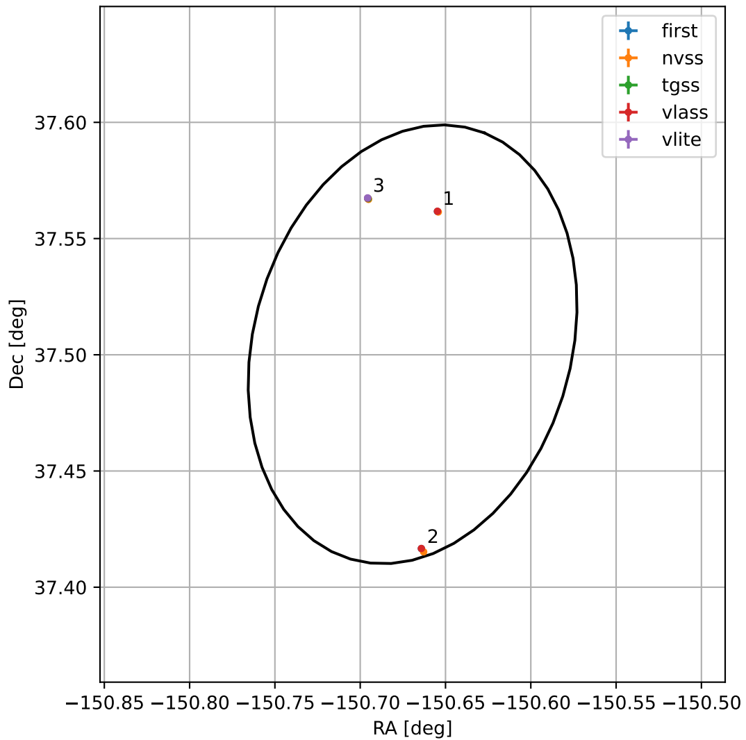
4FGL J1357.3+3730
