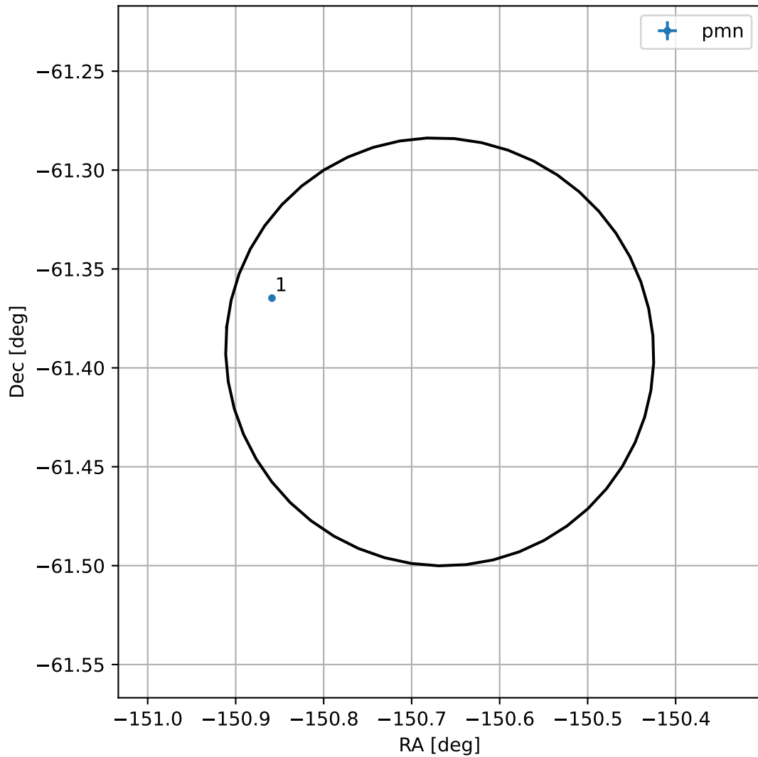
4FGL J1357.3-6123
