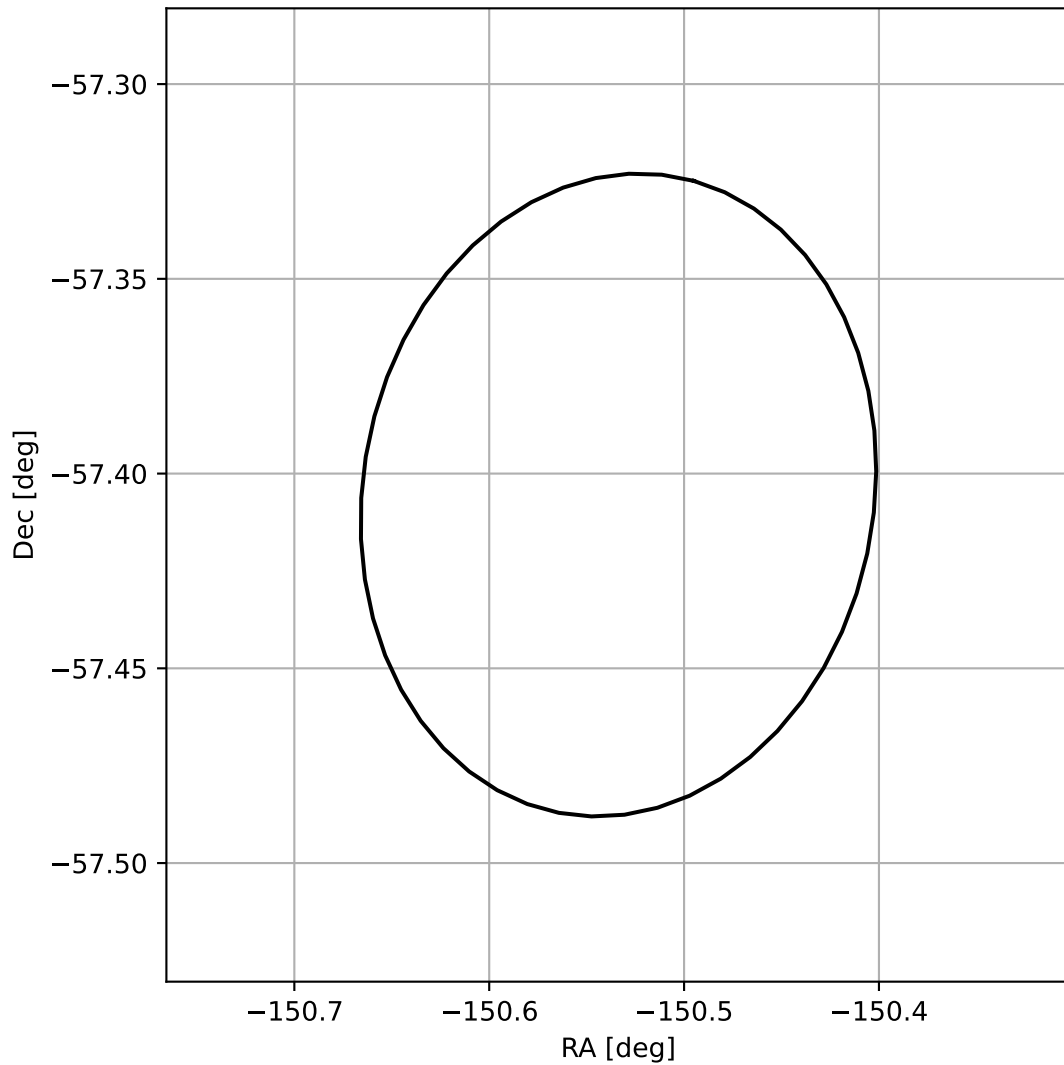
4FGL J1357.8-5724
