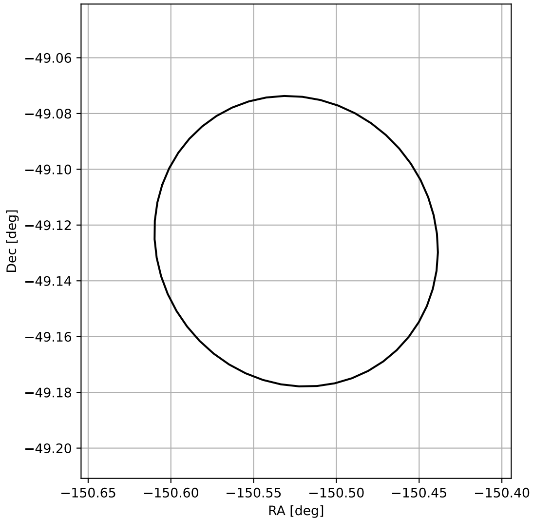
4FGL J1357.9-4907
