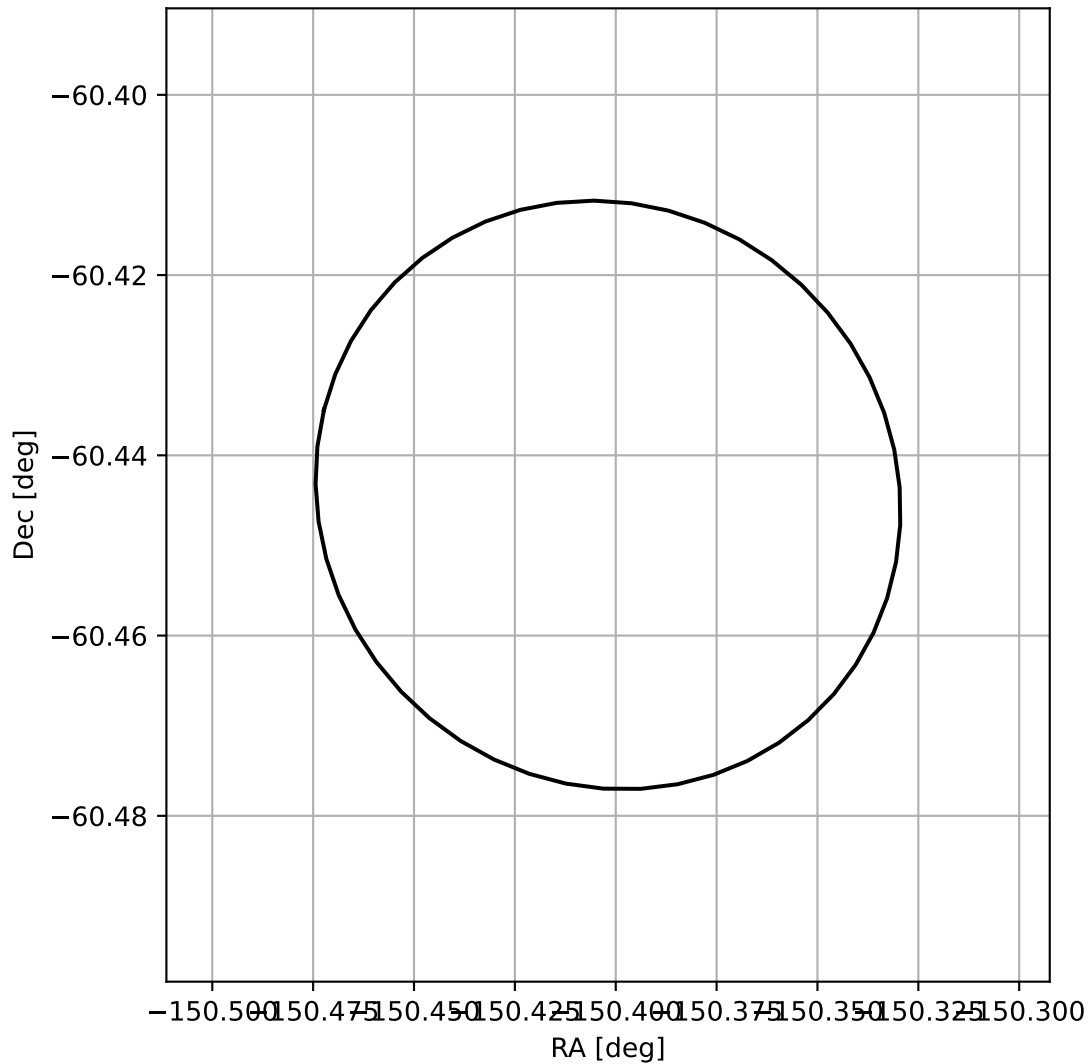
4FGL J1358.3-6026
