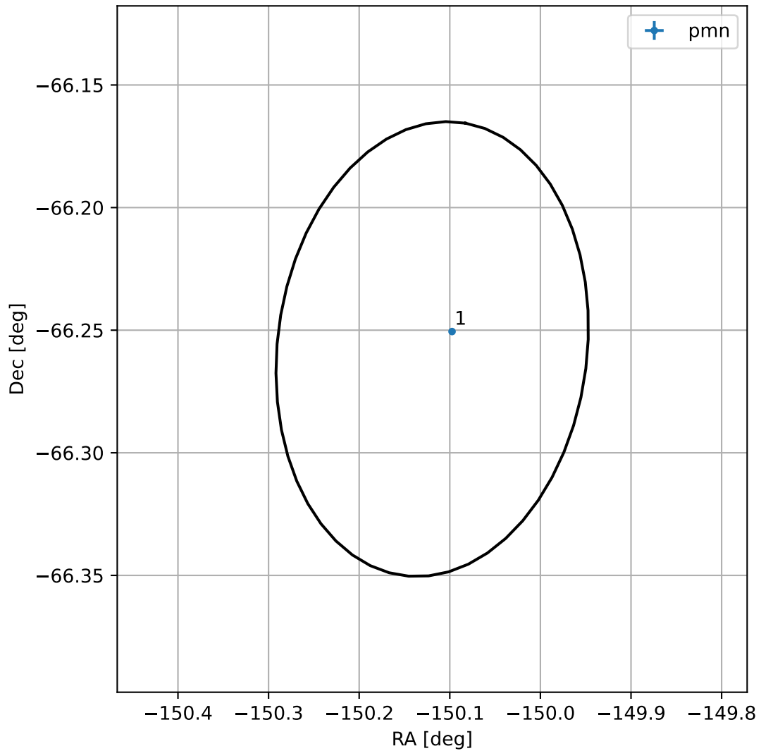
4FGL J1359.5-6615
