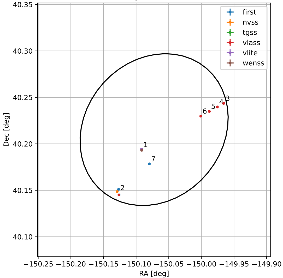
4FGL J1359.7+4012
