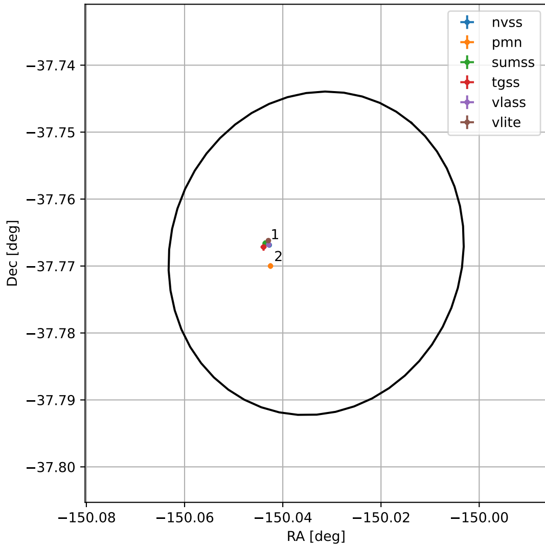
4FGL J1359.8-3746
