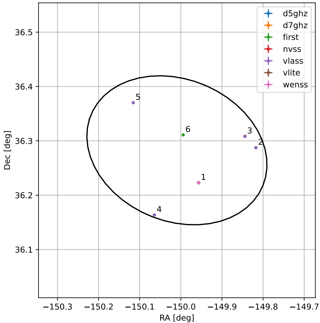
4FGL J1359.9+3616
