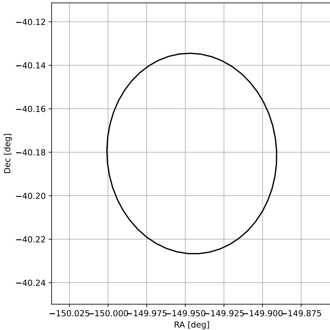
4FGL J1400.2-4010
