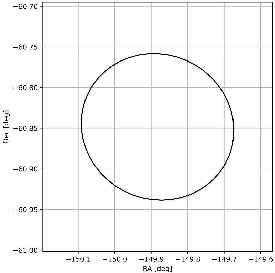
4FGL J1400.4-6050
