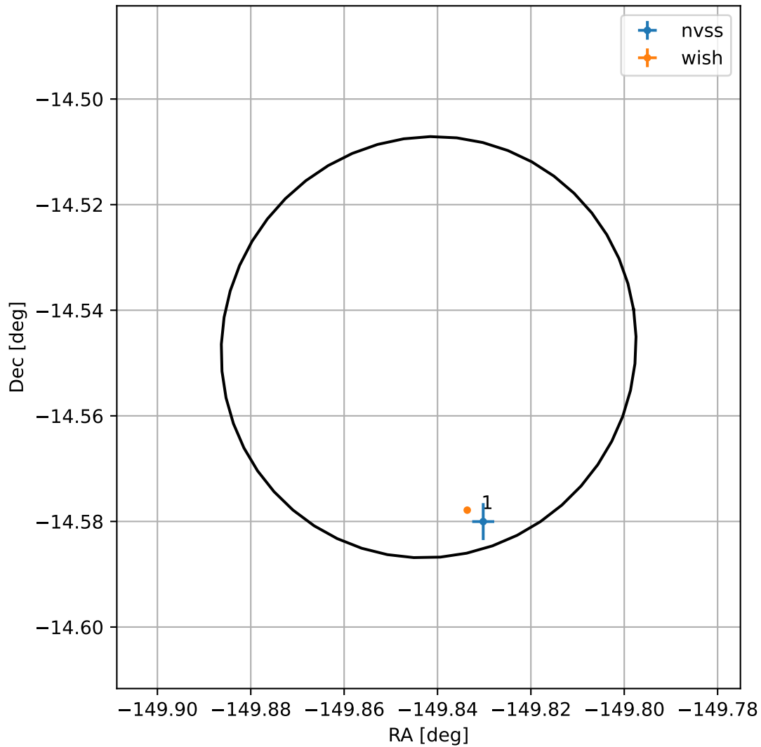
4FGL J1400.6-1432
