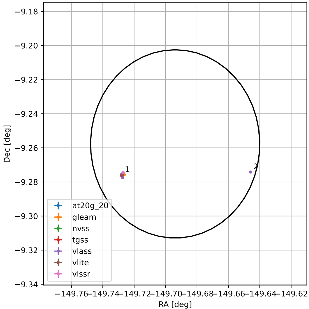
4FGL J1401.2-0915
