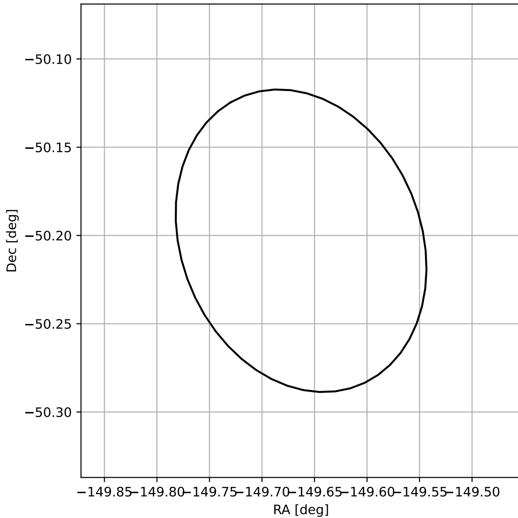
4FGL J1401.3-5012
