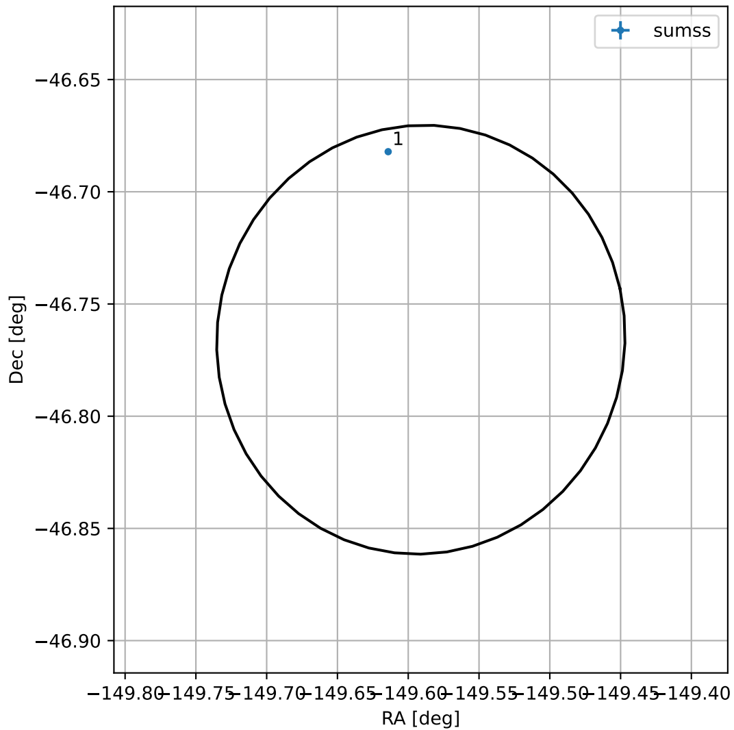
4FGL J1401.6-4645
