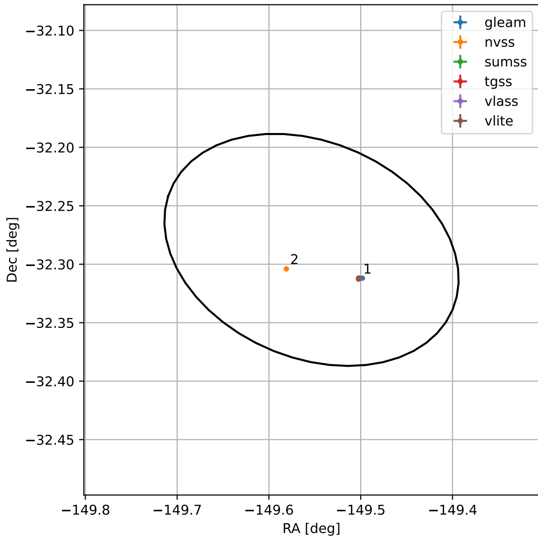
4FGL J1401.7-3217
