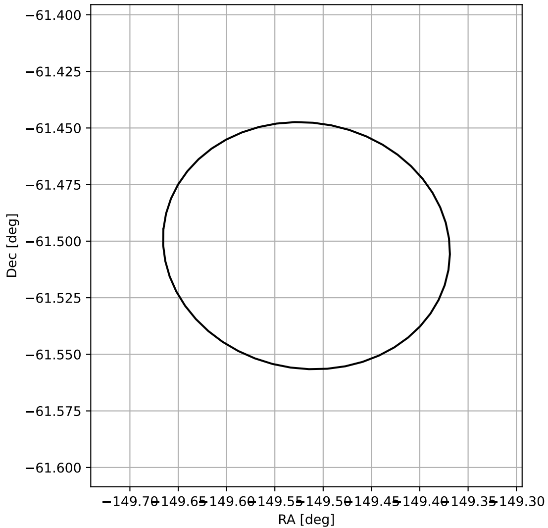
4FGL J1401.9-6130
