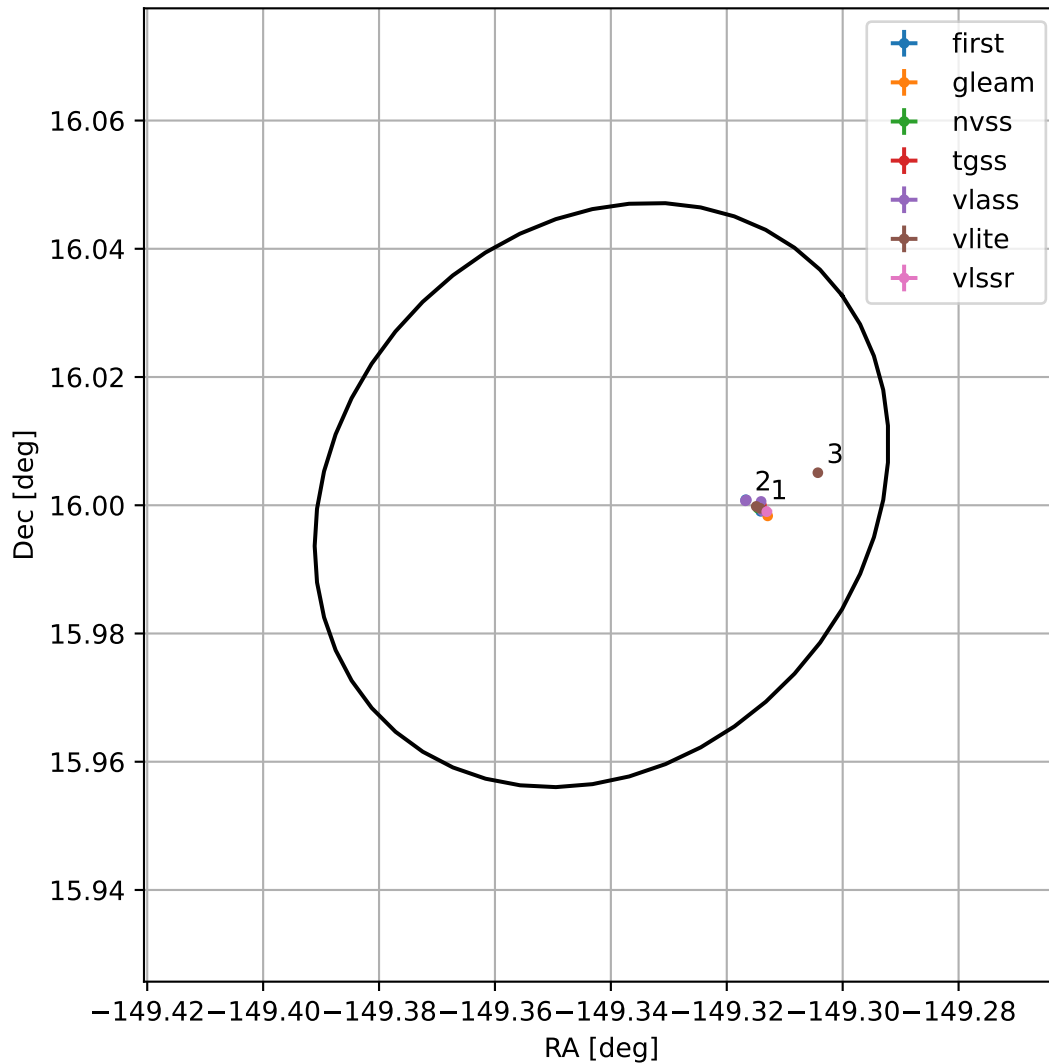
4FGL J1402.6+1600
