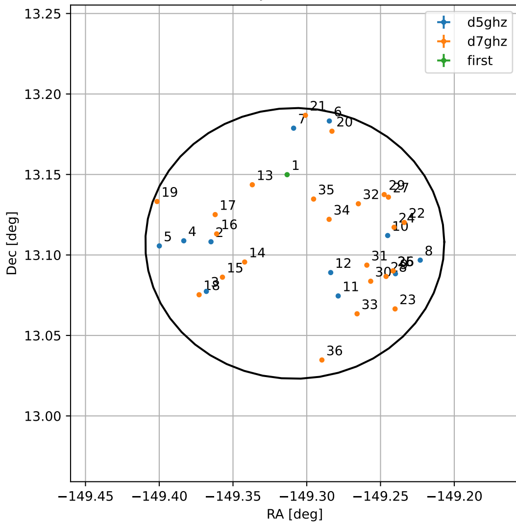
4FGL J1402.7+1306
