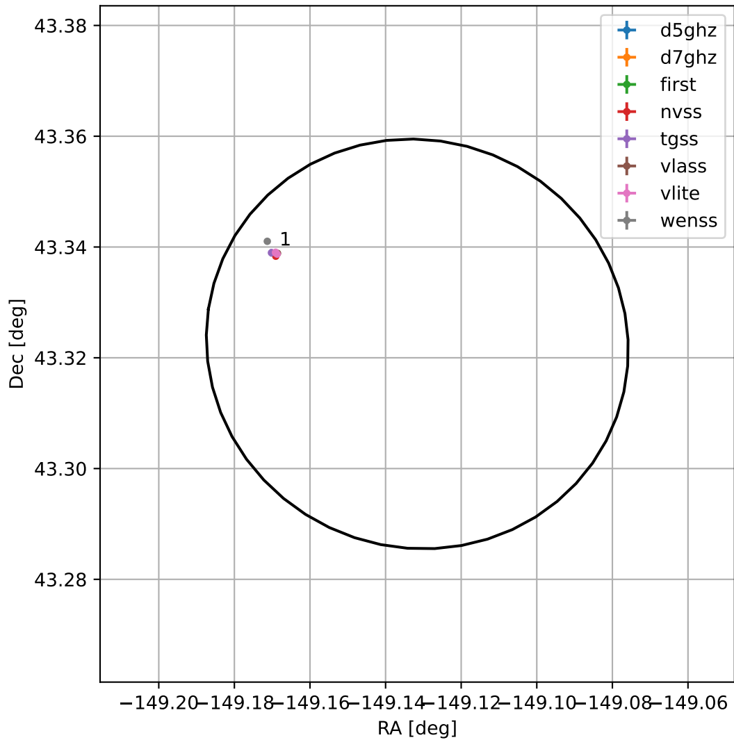
4FGL J1403.4+4319
