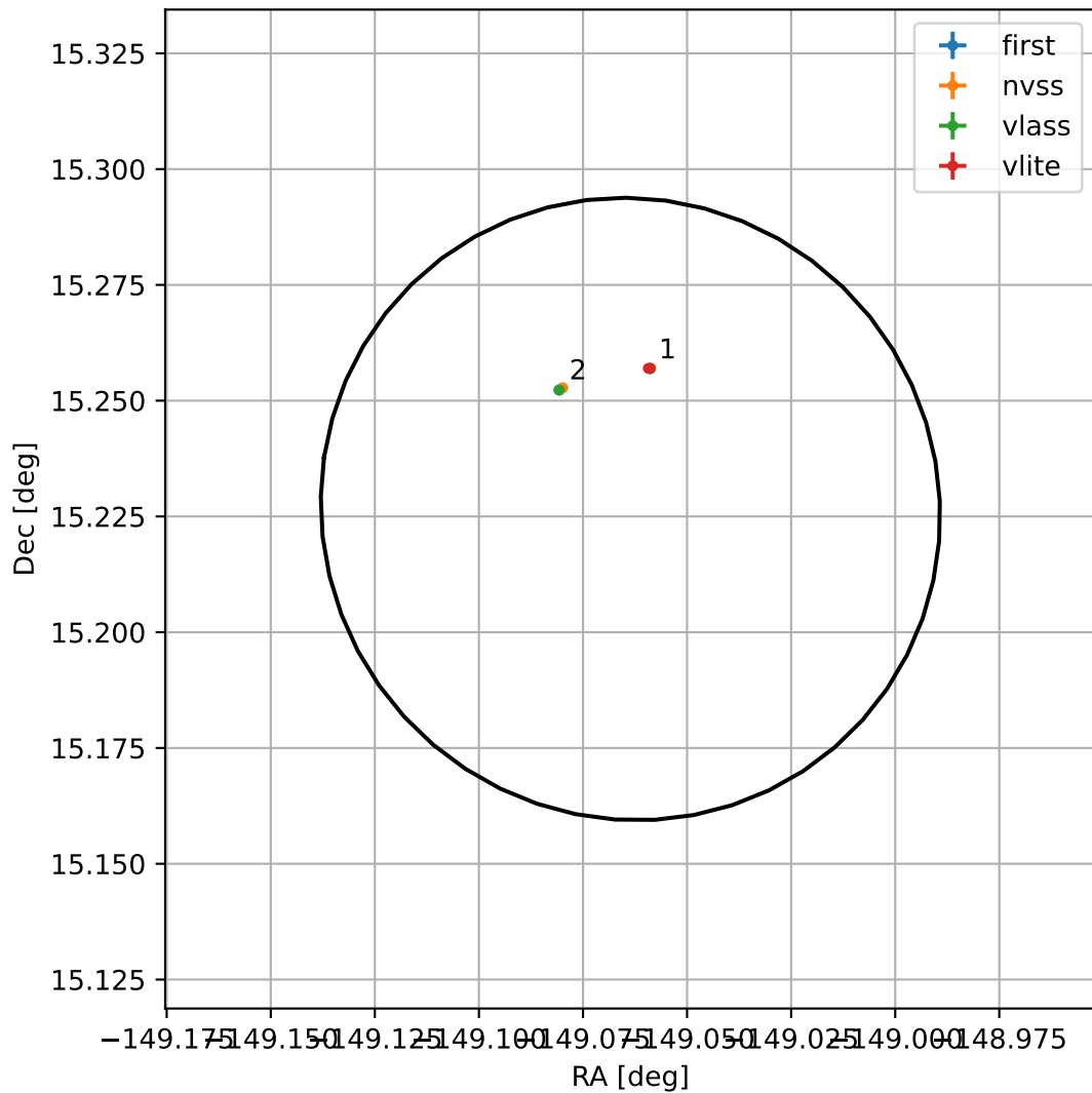
4FGL J1403.7+1513
