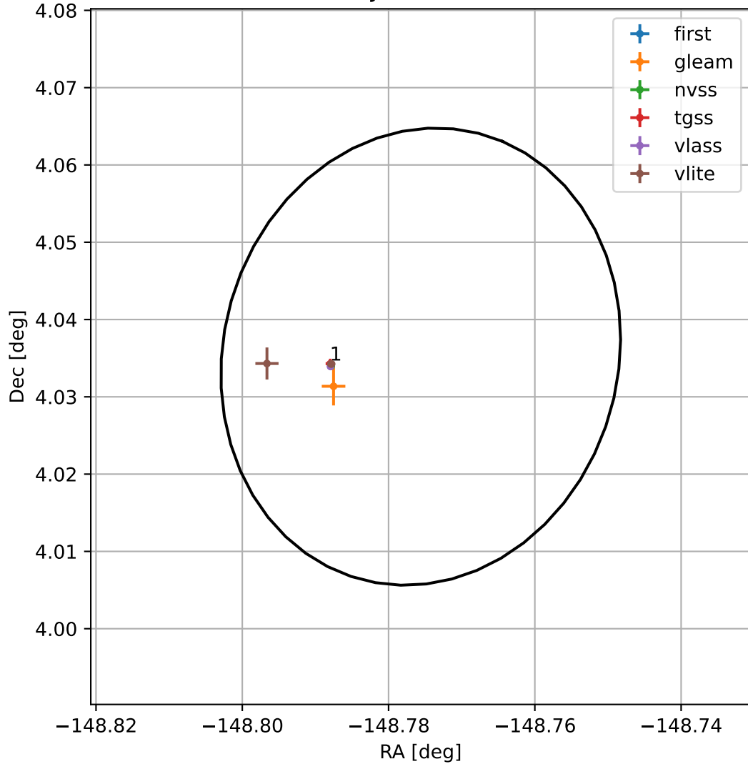
4FGL J1404.8+0402
