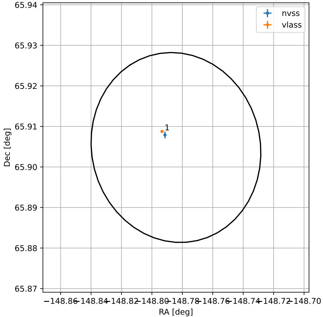
4FGL J1404.8+6554
