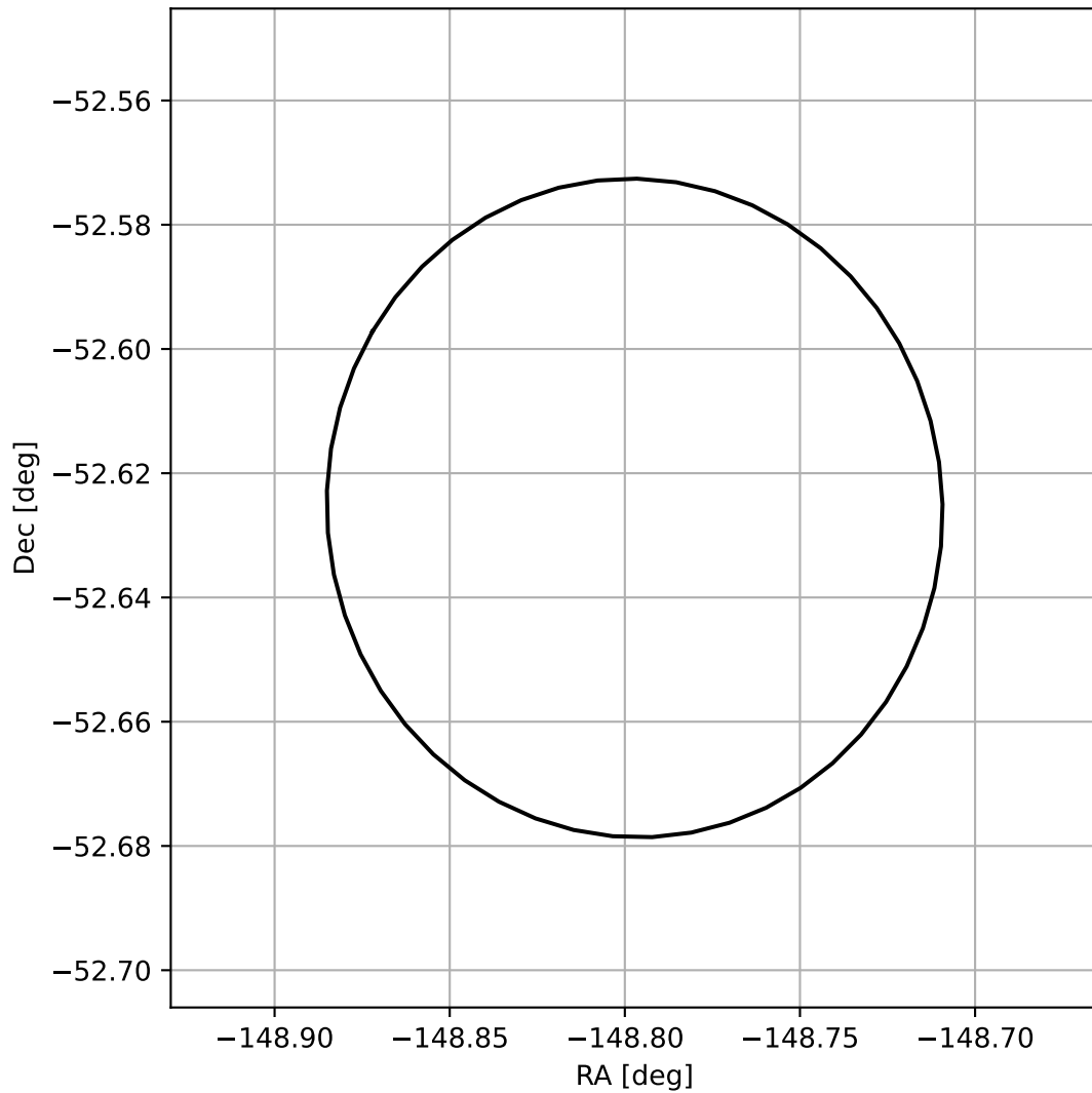
4FGL J1404.8-5237
