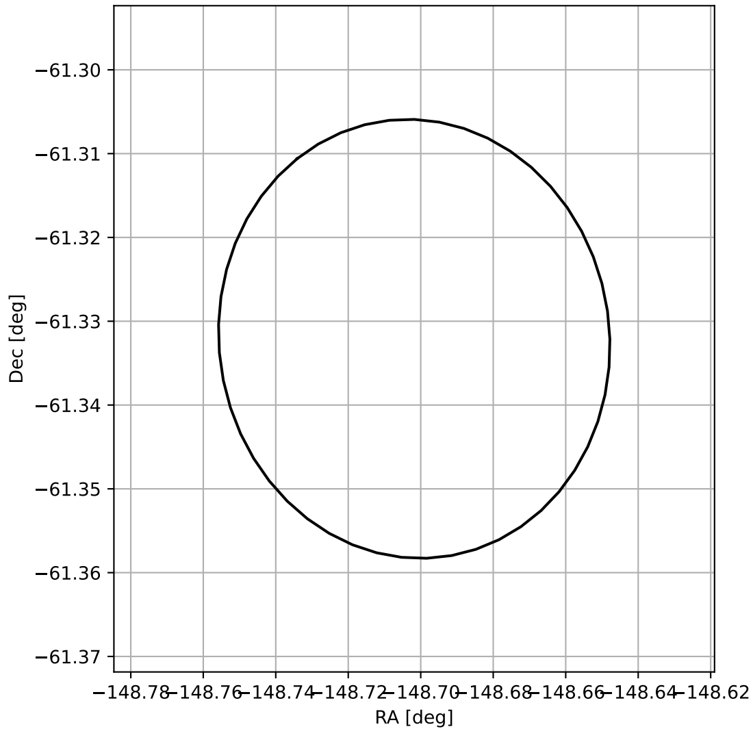
4FGL J1405.1-6119
