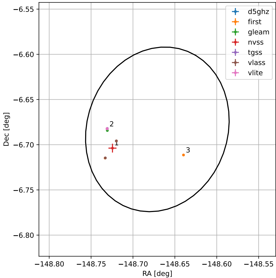
4FGL J1405.3-0640
