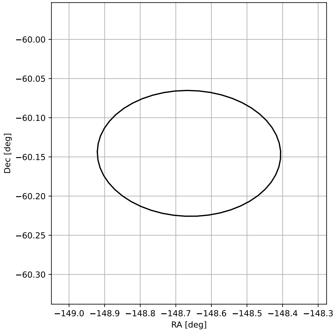
4FGL J1405.3-6008
