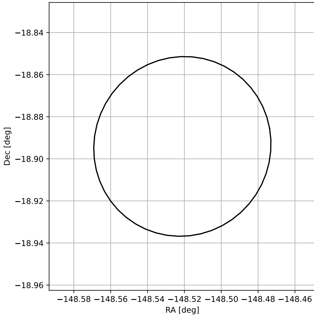
4FGL J1405.9-1853
