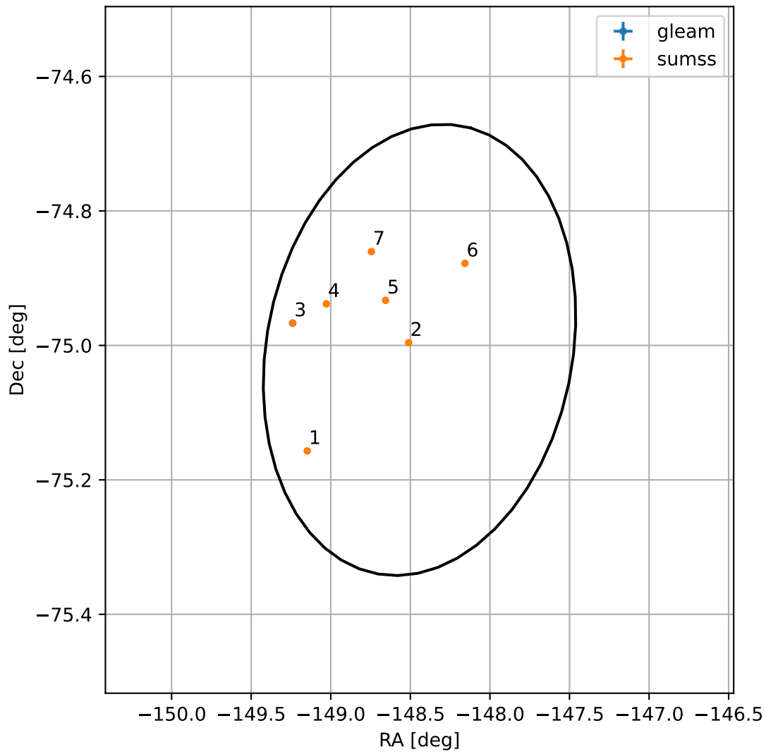
4FGL J1406.2-7500
