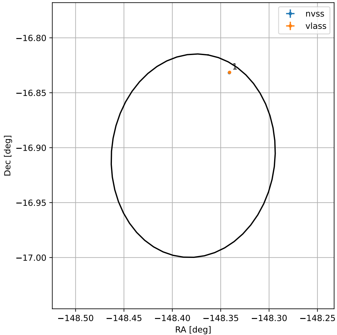
4FGL J1406.4-1654
