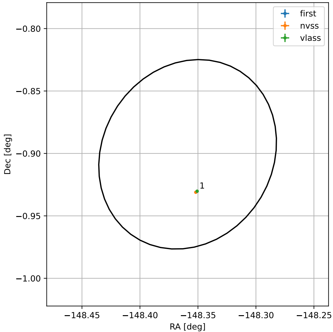
4FGL J1406.5-0054
