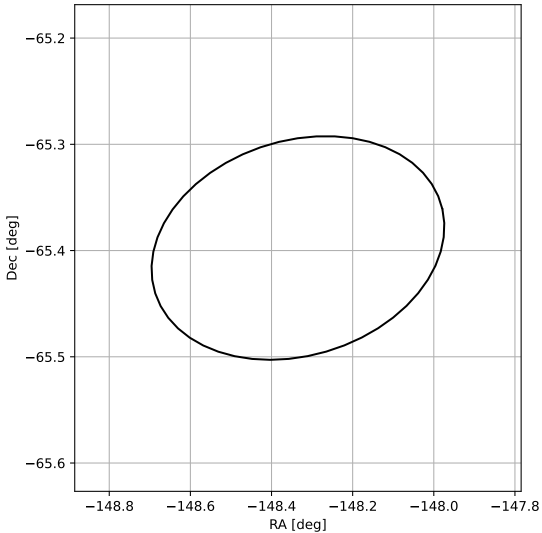
4FGL J1406.6-6523
