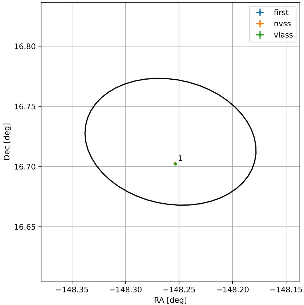
4FGL J1406.9+1643
