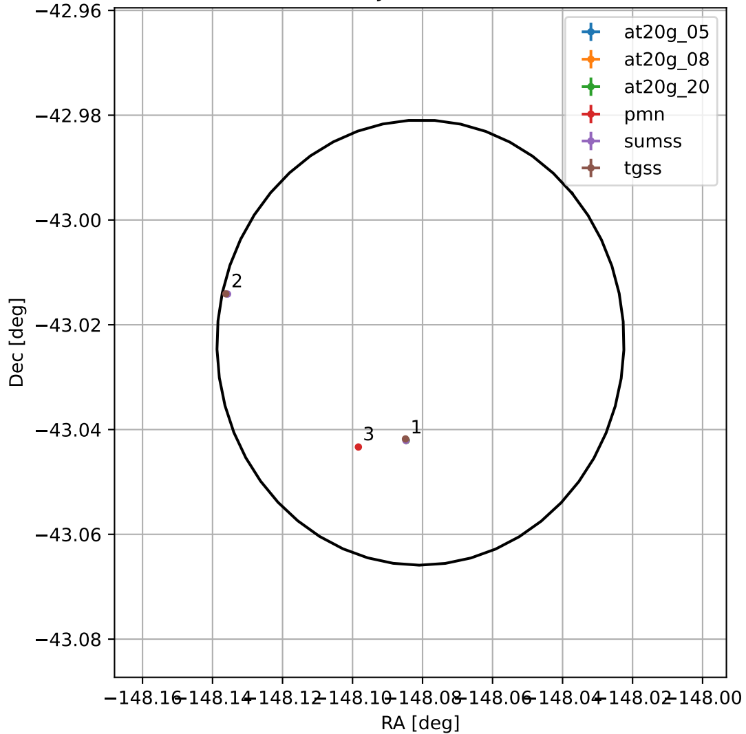
4FGL J1407.6-4301
