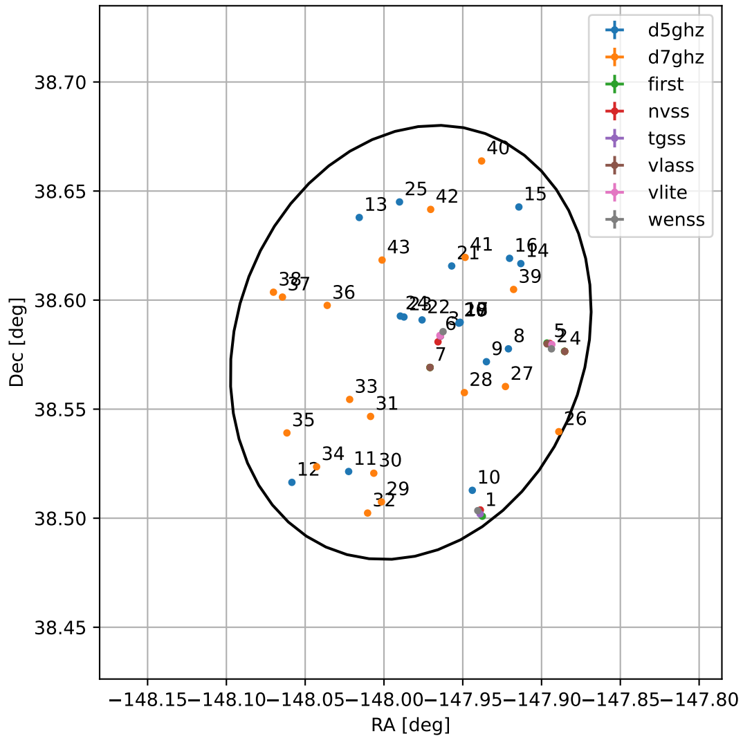
4FGL J1408.0+3834
