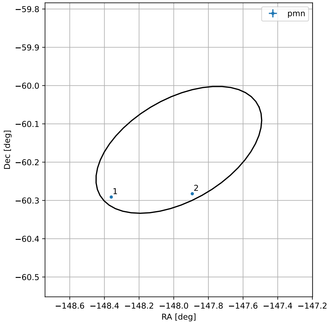
4FGL J1408.1-6010
