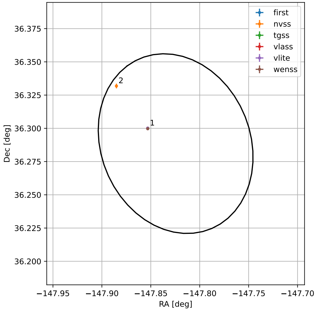
4FGL J1408.7+3617
