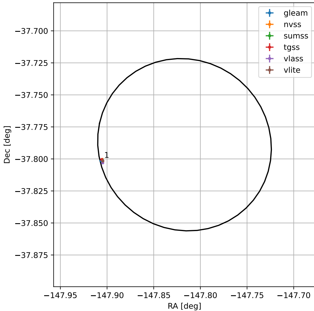
4FGL J1408.7-3747
