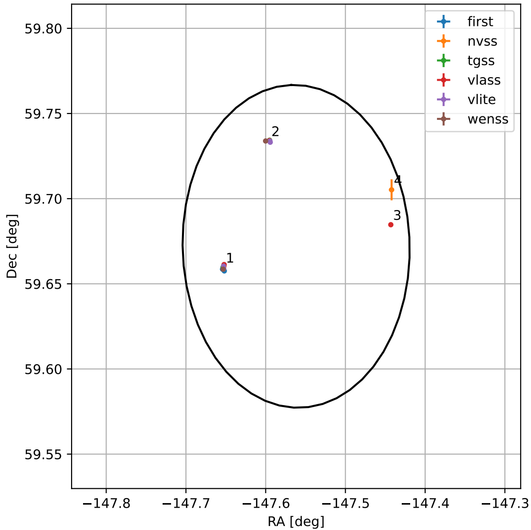
4FGL J1409.7+5940
