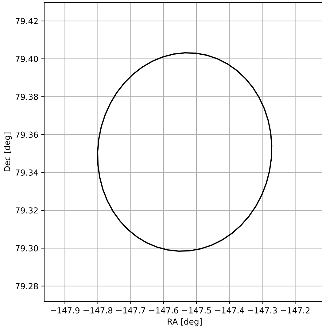
4FGL J1409.8+7921
