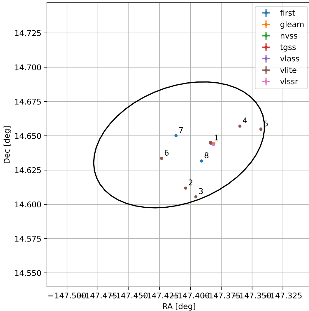
4FGL J1410.3+1438
